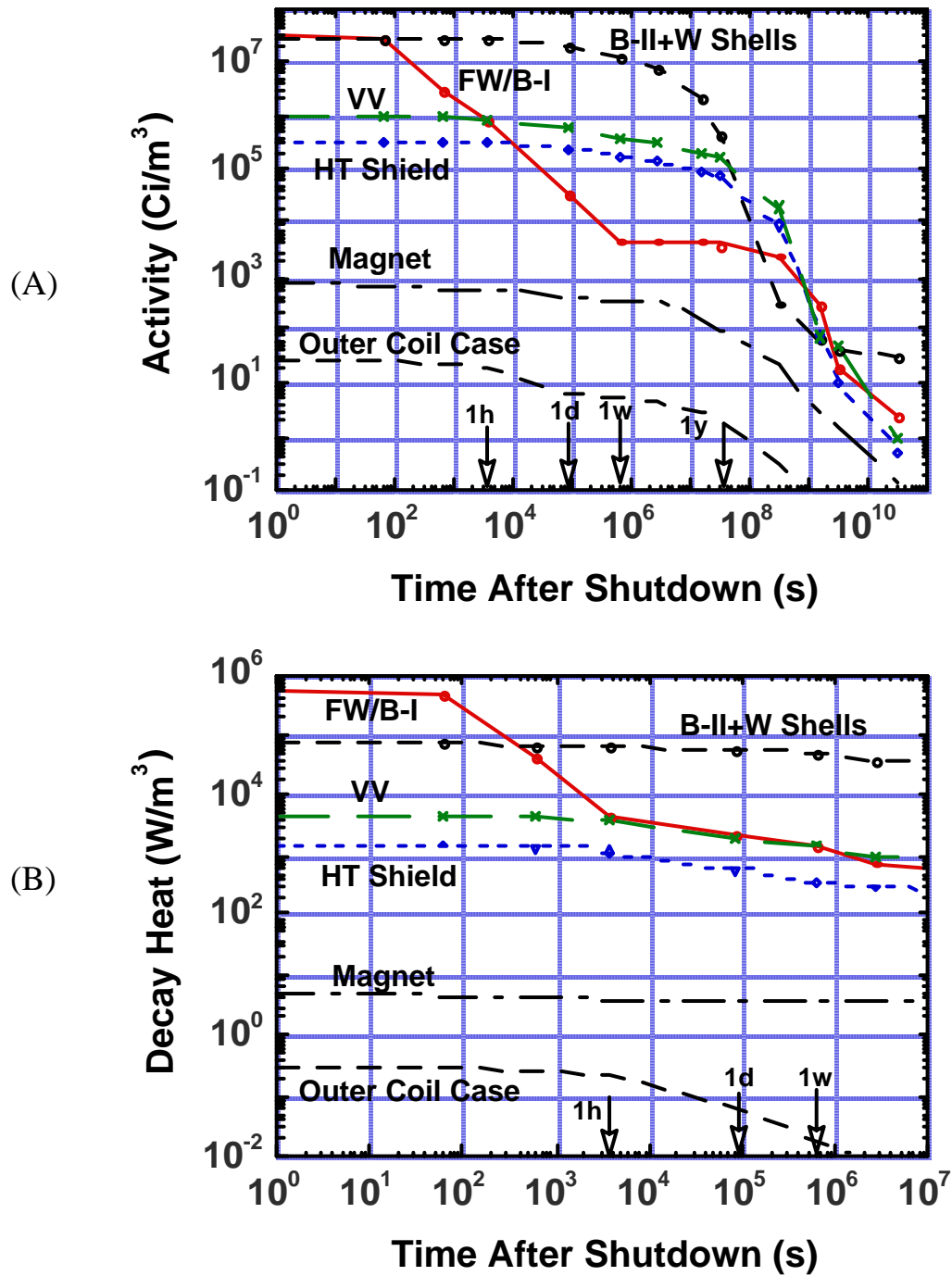
Fig. 10. Specific activity (A) and decay heat (B) on the outboard components of ARIES-AT.
