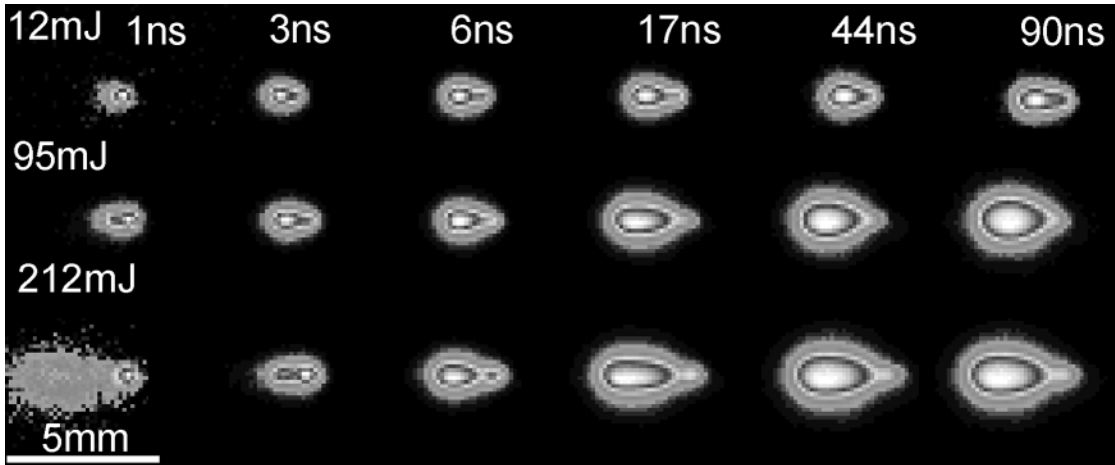
FIG. 3. ICCD photographs of the time evolution of visible emission from a laser-produced argon spark at different laser energies. The experimental parameters are the same as described in Fig. 2. All of the images are normalized to their maximum intensity.
