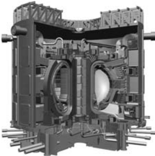
Fig. 2. The ITER facility, presently in international negotiation, is designed to integrate magnetic fusion burning plasma physics with fusion technologies, producing hundreds of megawatts of fusion power for long pulses.
