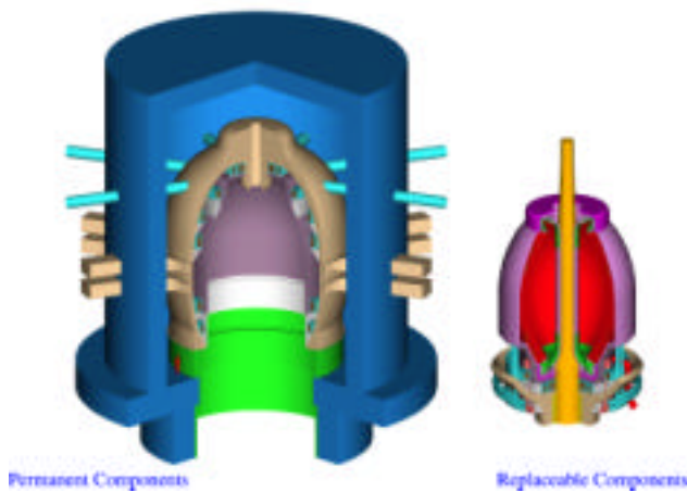
Fig.2. Solid model of the ARIES-ST power core, showing permanent and replaceable components
