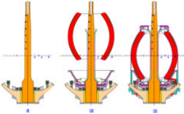
Fig.4. Power core assembly sequence
