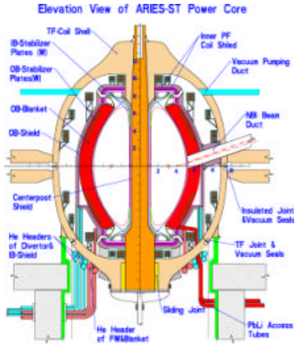
Fig.1. Elevation view of the ARIES-ST power core
