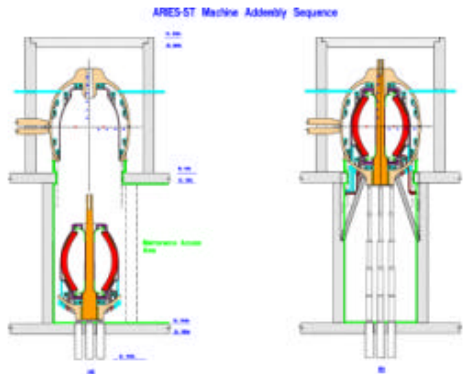
Fig.3. Power core maintenance paths
