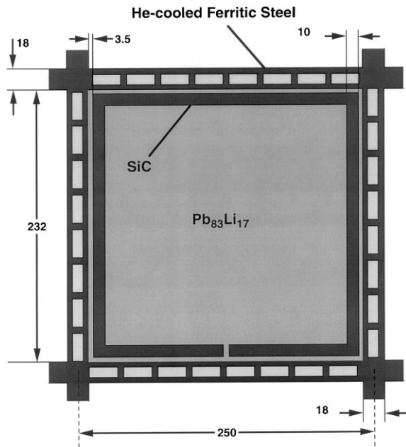
Fig. 4. Cross section of the breeder region unit cell.
