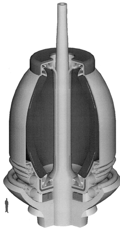
Fig. 2. Power core replacement unit.
