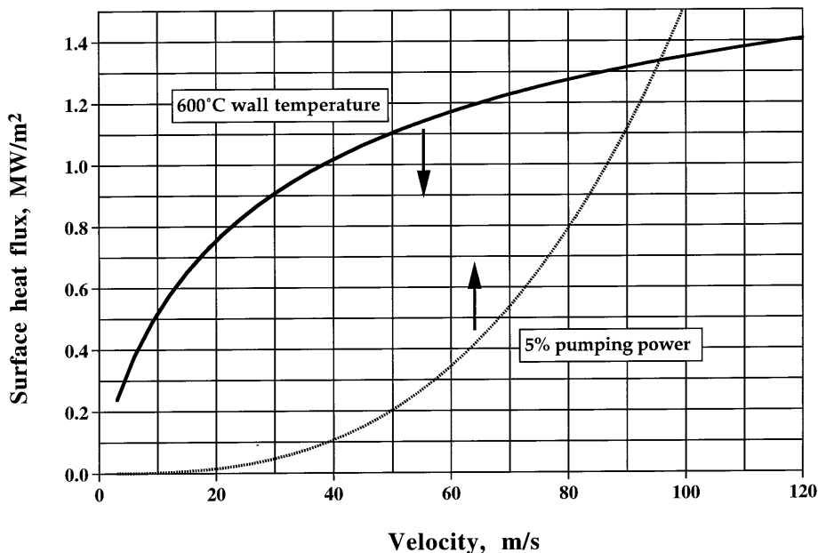
Fig. 5. Heat flux window of operation in the outboard first wall.
