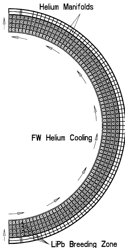
Fig. 3. Mid-plane outboard blanket horizontal cross-section.
