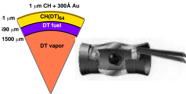
Fig. 1. Baseline direct and indirect drive target designs 5, 6 (not to scale)
