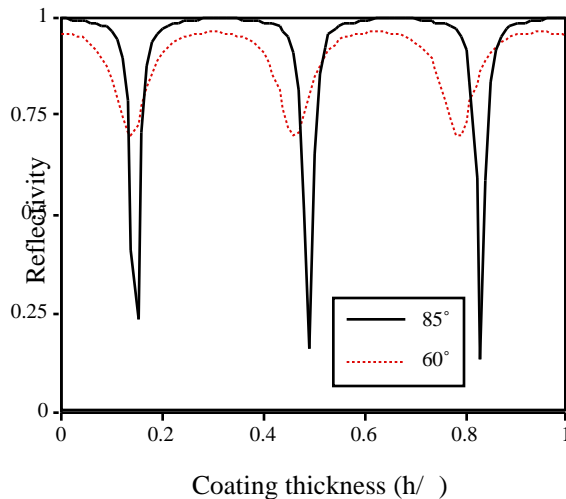
Fig. 8. Effect of surface oxide on Al reflectivity
