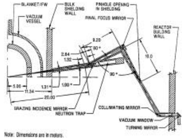
Fig. 7. Layout of final optic 1
