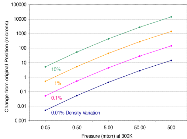
Fig. 5. Uncertainties in chamber gas pressure will lead to significant perturbations in target trajectory.
