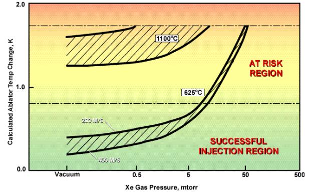
Fig. 4. Successful injection of direct drive targets requires control of heating from the chamber walls and gas.
