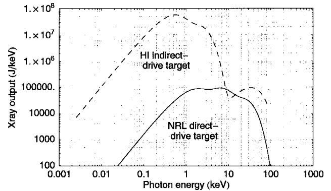
Fig. 2. Photon spectra.
